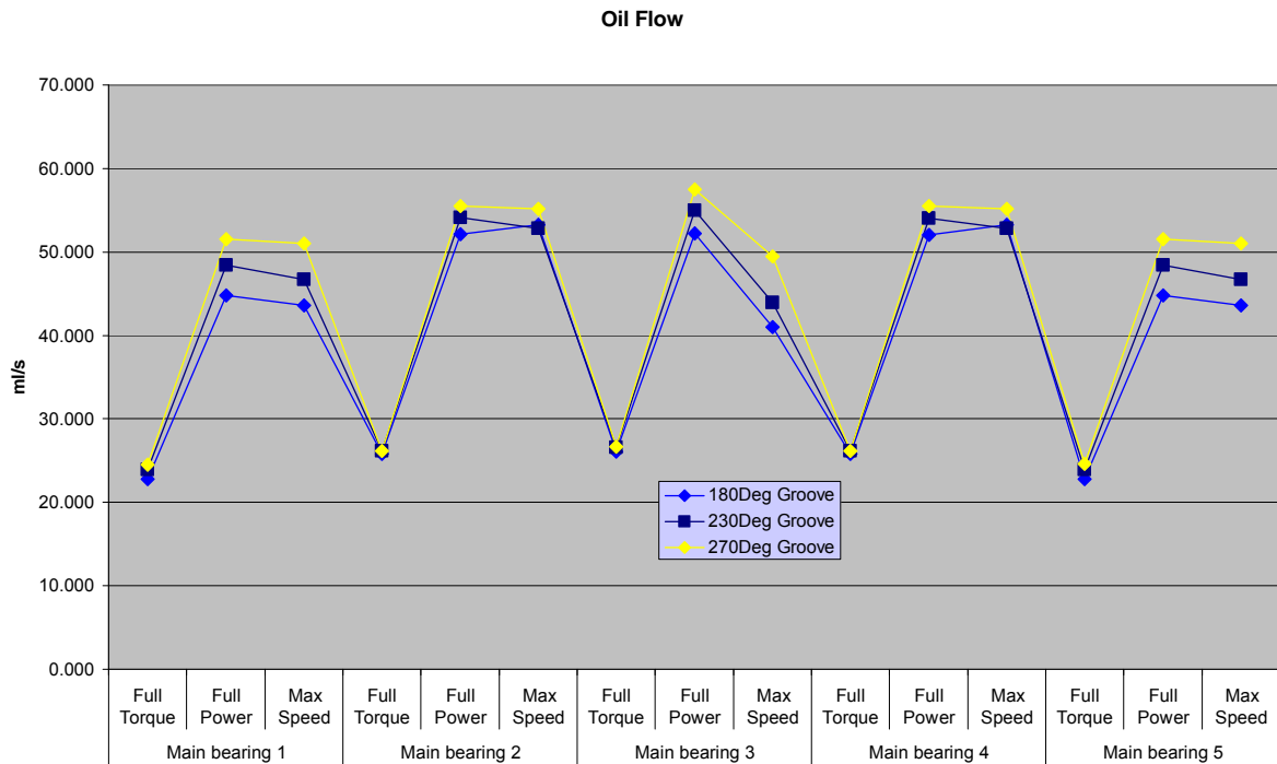
Fig. 3 – Oil Flow
