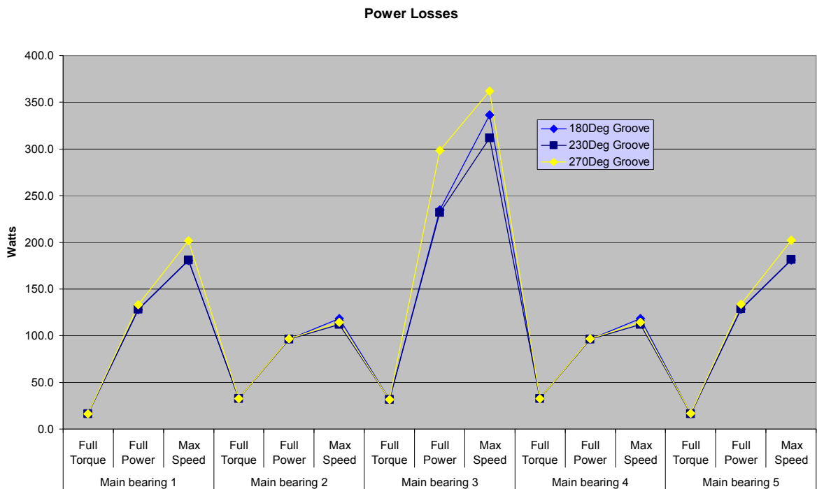
Fig. 4 – Power Loss
